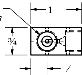
LEFT VIEW
