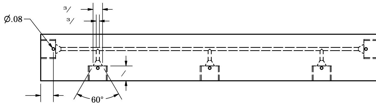
TOP VIEW
